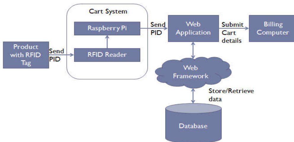
Figure 1: System Architecture of overall project
