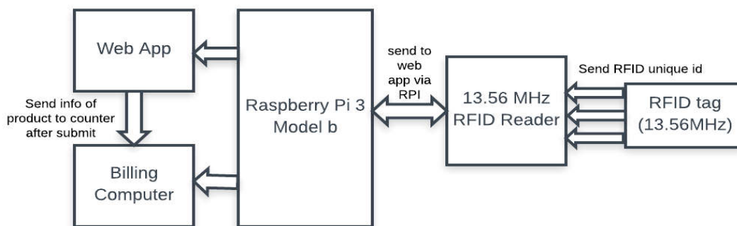
Figure 2: Block Diagram of Interfacing Units
